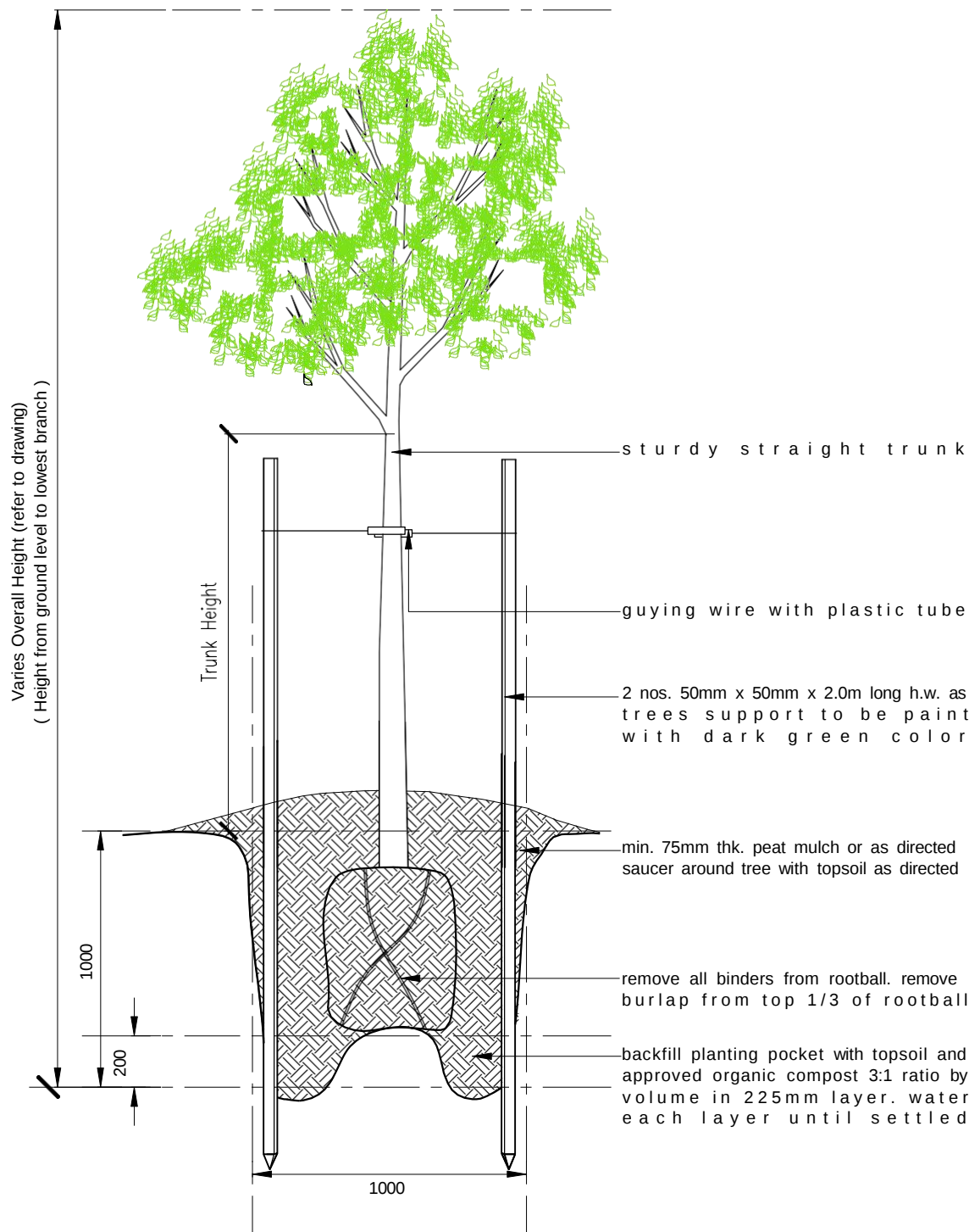
PLANTING DETAIL (SHADES TREE) NOT TO SCALE
