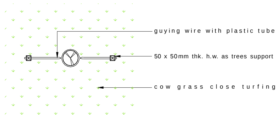
PLAN OF TREES SUPPORT NOT TO SCALE
