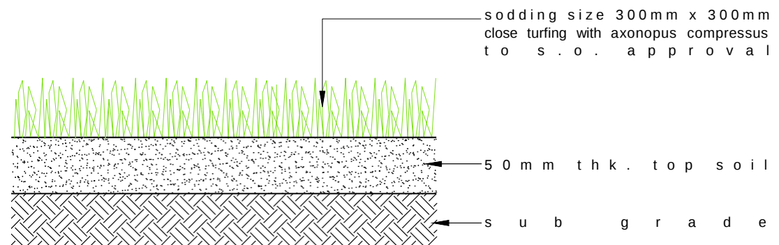
PLANTING DETAIL OF TURFING NOT TO SCALE
