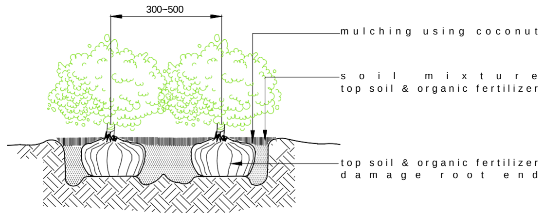
PLANTING DETAIL (SHRUB) NOT TO SCALE
